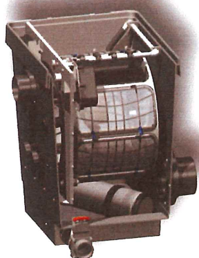
Trumfiltermodul
